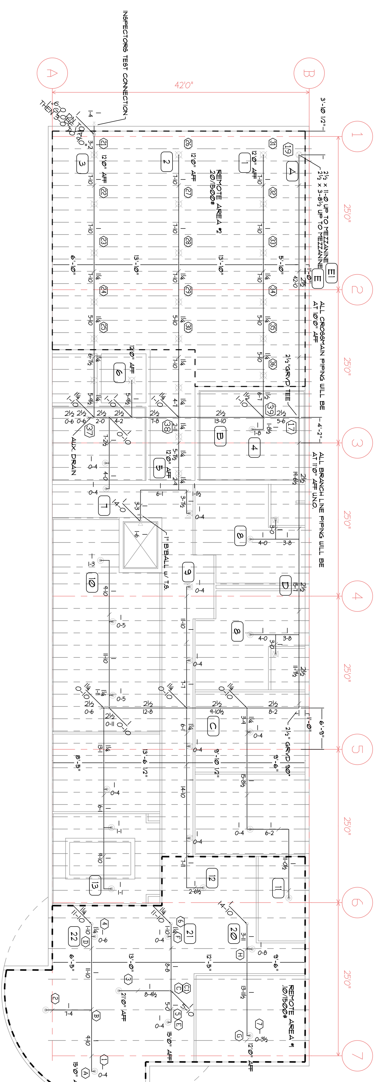
OFFICE AREA FIRE PROTECTION PLAN SCALE: 1/8" = 1'-0"
